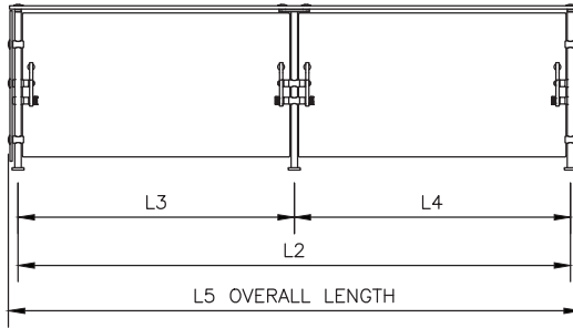
Front: -EQ, -OF and -96 Models
