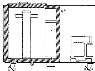
SECTIONAL VIEW
