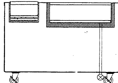
SECTIONAL VIEW
