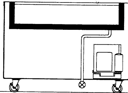
SECTIONAL VIEW
