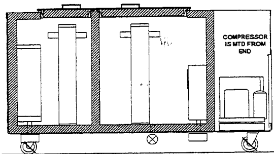
SECTIONAL VIEW
